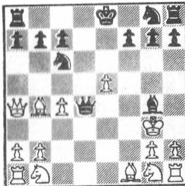
61 After 11 Kg3
